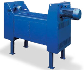
PHS-O shredder Feeding via conveyor belt
